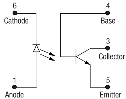
Figure 1. OLS449 Block Diagram
