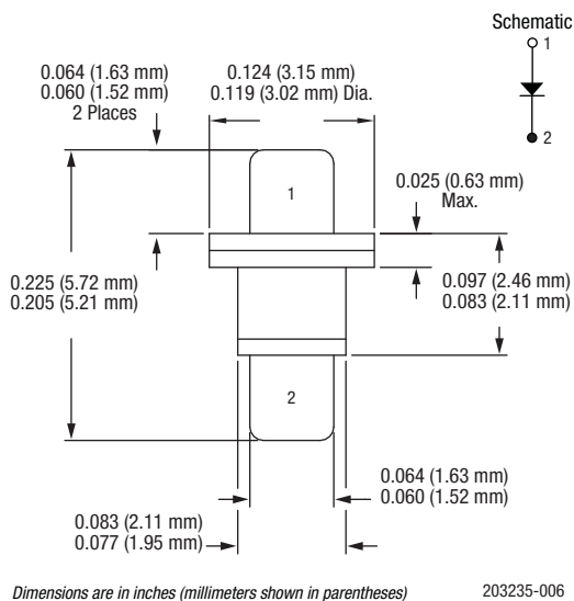
Figure 6. -210 Package
