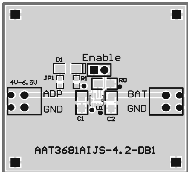
Figure 5: AAT3681A Evaluation Board Top Side Layout.
