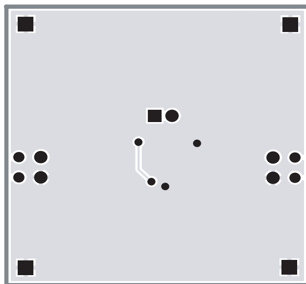
Figure 6: AAT3681A Evaluation Board Bottom Side Layout.
