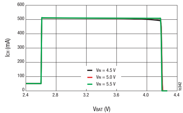
Figure 4. Charge Current vs Battery Voltage ( R_{SET} = 3.24\text{ k}\Omega )
