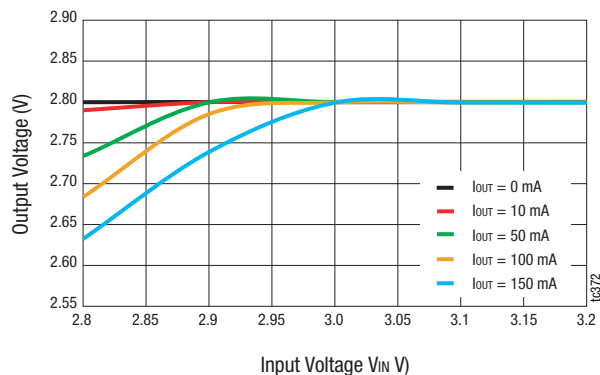
Figure 34. Dropout Characteristics vs Input Voltage ( V_{OUT} = 2.8 \text{ V} )
