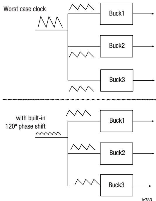
Figure 45. Buck Converter Phase Shifting
