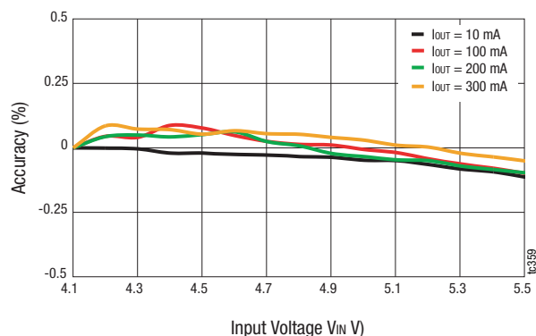
Figure 21. Buck 2 Line Regulation ( V_{OUT} = 1.8\text{ V} )
