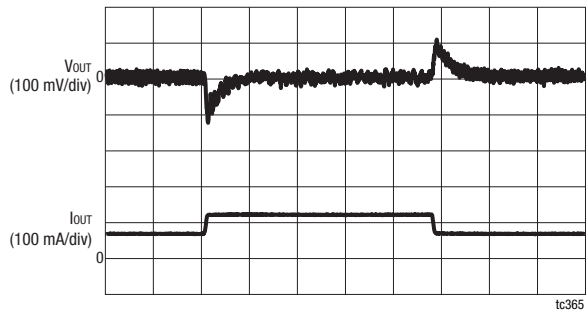
Figure 27. Buck 2 Load Transient Response ( V_{IN} = 5.0\text{ V} , V_{OUT} = 1.8\text{ V} , 75 mA to 125 mA Load)
