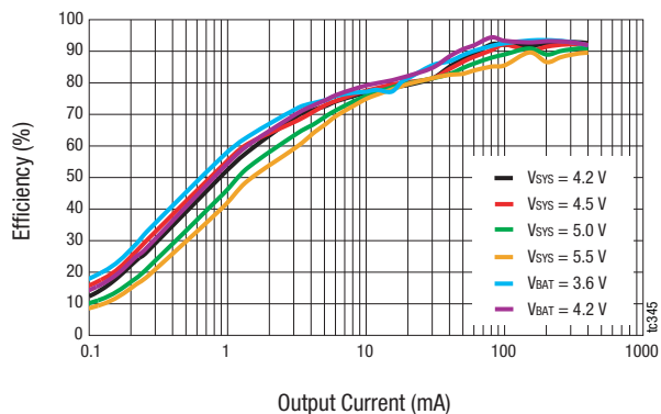
Figure 7. Step-Down Buck Efficiency vs Output Current ( V_{out} = 3.0\text{ V} , L = 2.2\text{ }\mu\text{H} )
