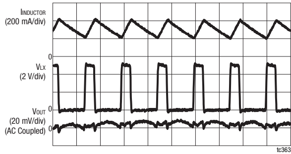
Figure 25. Buck 3 Output Ripple ( V_{IN} = 5.0\text{ V} , V_{OUT} = 1.2\text{ V} , C_{OUT} = 4.7\text{ }\mu\text{F} , 300 mA Load)
