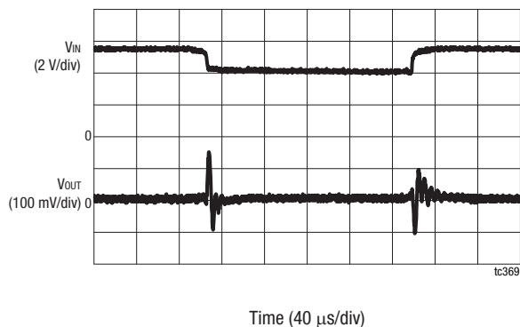
Figure 31. Buck 3 Line Transient Response ( V_{IN} = 4.1 \text{ V} to 5.0 \text{ V} , V_{OUT} = 1.2 \text{ V} , 300 \text{ mA} Load)
