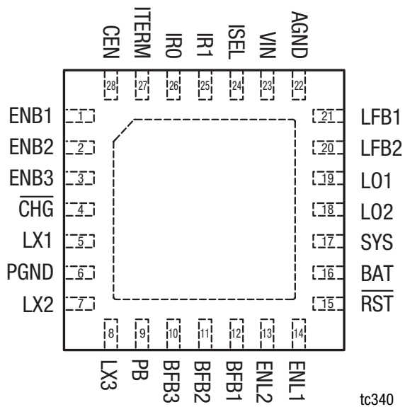
Figure 2. AAT3607 Pinout – 28-Pin, 4 mm × 4 mm TQFN (Top View)
