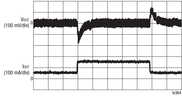
Figure 26. Buck 1 Load Transient Response ( V_{IN} = 5.0\text{ V} , V_{OUT} = 3.0\text{ V} , 75 mA to 150 mA Load)
