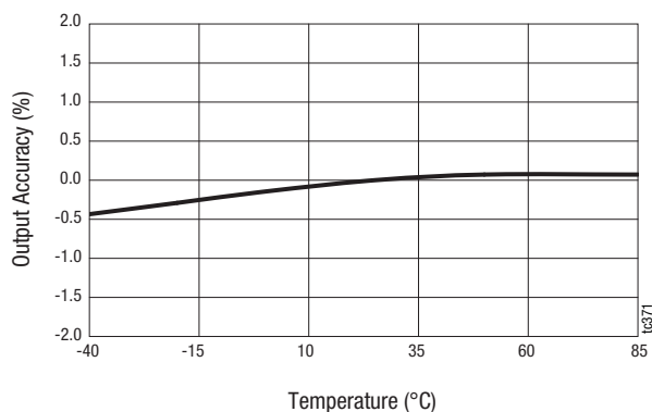
Figure 33. Output Voltage Accuracy vs. Temperature ( V_{IN} = 5.0 \text{ V} , V_{OUT} = 2.8 \text{ V} , I_{OUT} = 150 \text{ mA} )
