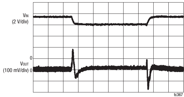
Figure 29. Buck 1 Line Transient Response ( V_{IN} = 4.1\text{ V} to 5.0\text{ V} , V_{OUT} = 3.0\text{ V} , 400 mA Load)
