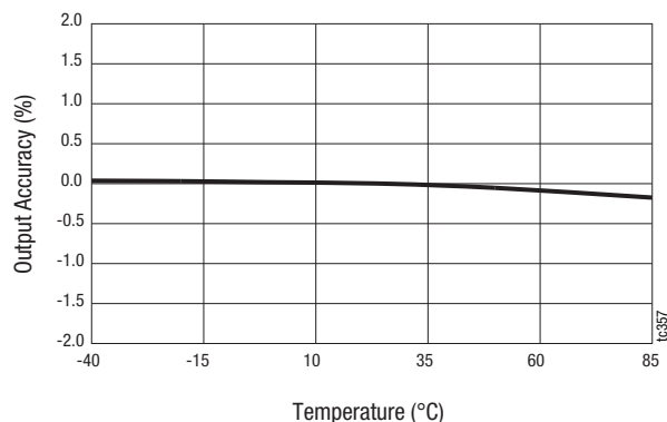
Figure 19. Buck 3 Output Voltage Accuracy vs Temperature ( V_{IN} = 5.0\text{ V} , V_{OUT} = 1.2\text{ V} , I_{OUT} = 300\text{ mA} )
