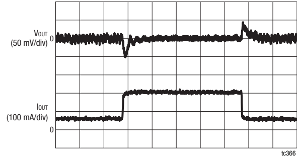
Figure 28. Buck 3 Load Transient Response ( V_{IN} = 5.0\text{ V} , V_{OUT} = 1.2\text{ V} , 75 mA to 200 mA Load)
