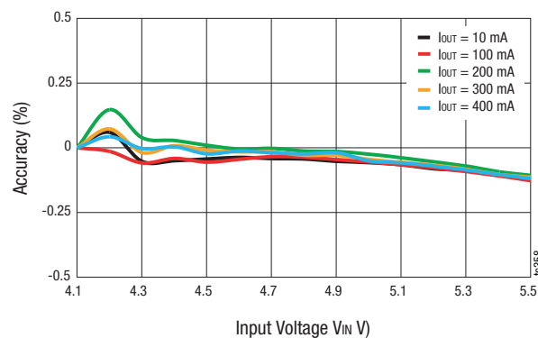
Figure 20. Buck 1 Line Regulation ( V_{OUT} = 3.0\text{ V} )
