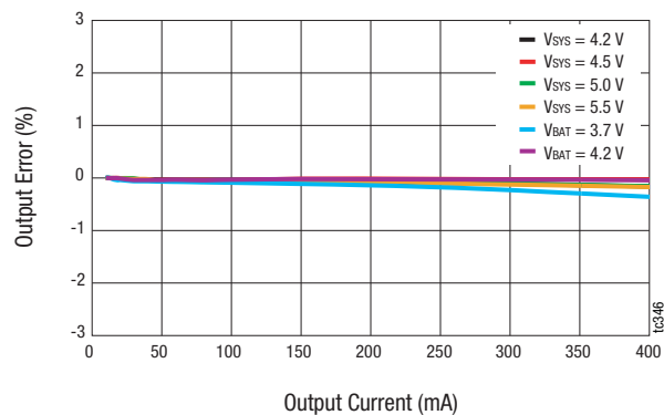
Figure 8. Buck 1 DC Regulation ( V_{out} = 3.0\text{ V} , L = 2.2\text{ }\mu\text{H} )
