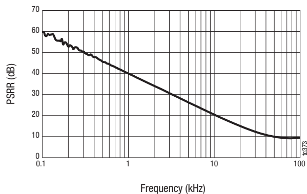
Figure 35. PSRR vs Frequency ( V_{IN} = 5.0 \text{ V} , V_{RIPPLE} = 500 \text{ mV} , 10 \text{ mA} Load)
