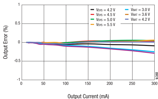
Figure 10. Buck 2 DC Regulation ( V_{out} = 1.8\text{ V} , L = 2.2\text{ }\mu\text{H} )
