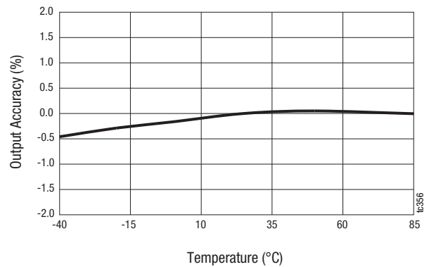
Figure 18. Buck 2 Output Voltage Accuracy vs Temperature (VIN = 5.0 V, VOUT = 1.8 V, IOUT = 300 mA)
