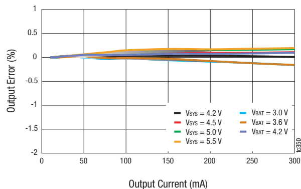
Figure 12. Buck 3 DC Regulation ( V_{out} = 1.2\text{ V} , L = 2.2\text{ }\mu\text{H} )
