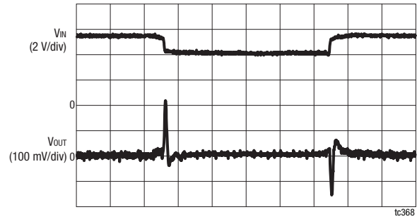
Figure 30. Buck 2 Line Transient Response ( V_{IN} = 4.1\text{ V} to 5.0\text{ V} , V_{OUT} = 1.8\text{ V} , 300 mA Load)
