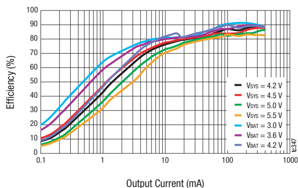
Figure 9. Step-Down Buck Efficiency vs Output Current ( V_{out} = 1.8\text{ V} , L = 2.2\text{ }\mu\text{H} )
