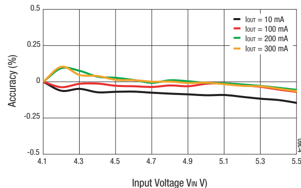
Figure 22. Buck 1 Line Regulation ( V_{OUT} = 1.2\text{ V} )
