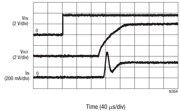
Figure 16. Buck 1 Soft Start (VIN = 5.0 V, VOUT = 3.0 V, IOUT = 400 mA)
