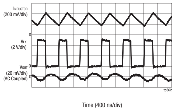
Figure 24. Buck 2 Output Ripple ( V_{IN} = 5.0\text{ V} , V_{OUT} = 1.8\text{ V} , C_{OUT} = 4.7\text{ }\mu\text{F} , 300\text{ mA Load} )
