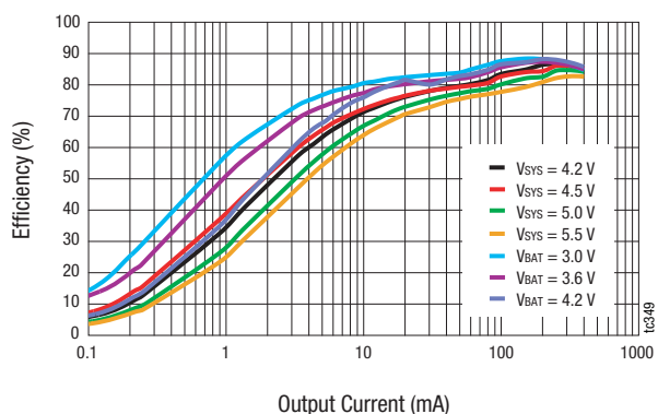
Figure 11. Step-Down Buck Efficiency vs Output Current ( V_{out} = 1.2\text{ V} , L = 2.2\text{ }\mu\text{H} )
