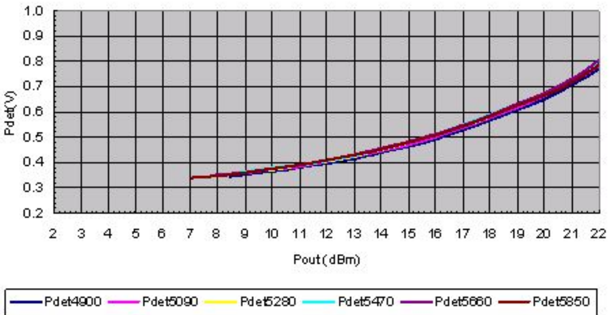
Figure 3: SE5007BT Power Detector Characteristic
