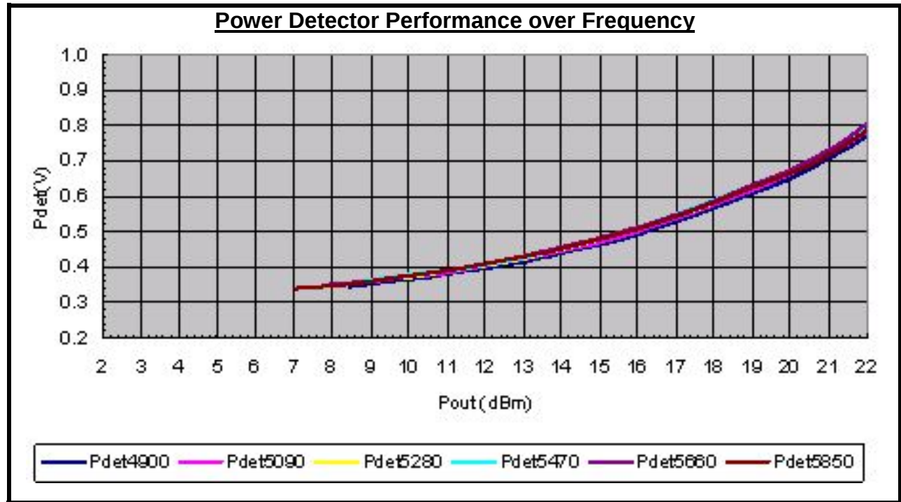
Figure 3: SE5007BT Power Detector Characteristic
