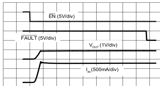
Start Into 1\Omega Load
