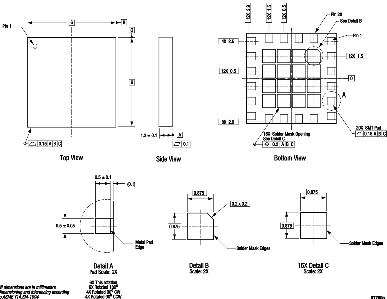
Figure 9. SKY65344-21 20-Pin MCM Package Dimensions
