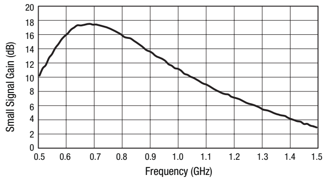
Figure 3. Small Signal Gain vs Frequency @ 25^{\circ}\text{C} ( P_{IN} = -20\ \text{dBm} )
