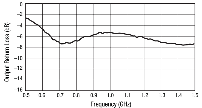
Figure 4. Output Return Loss vs Frequency @ 25^{\circ}\text{C} P_{IN} = -20\ \text{dBm}
