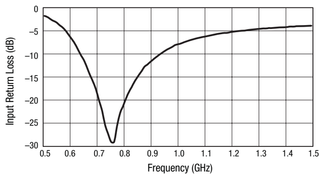
Figure 5. Input Return Loss vs Frequency @ 25^{\circ}\text{C} ( P_{IN} = -20\ \text{dBm} )
