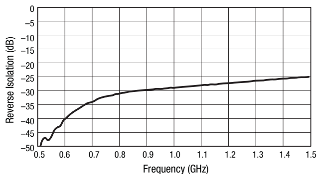
Figure 7. Reverse Isolation vs Frequency @ 25^{\circ}\text{C} ( P_{IN} = -20\ \text{dBm} )
