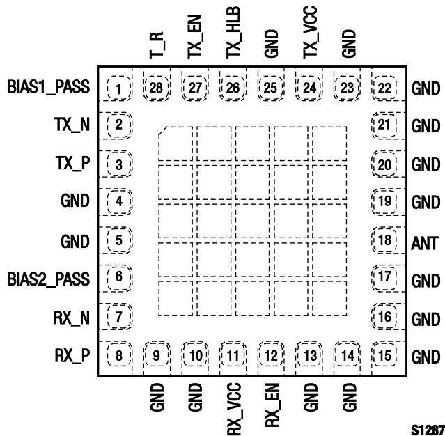
Figure 2. SKY65336-11 Pinout – 28-Pin MCM (Top View)
