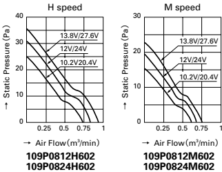
Air Flow and Static Pressure Characteristics (20mm thick)
