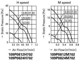
Air Flow and Static Pressure Characteristics (15mm thick)
