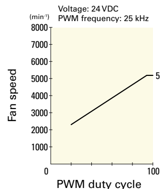
PWM duty - Speed characteristics example
