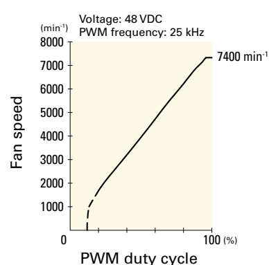
PWM duty - Speed characteristics example
