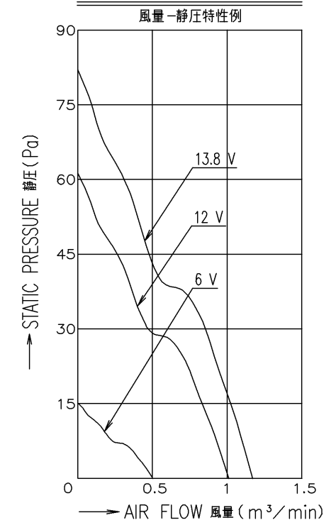
PERFORMANCE CURVES
