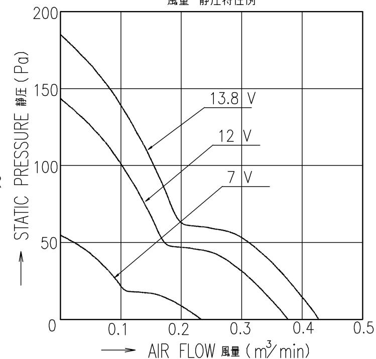
PERFORMANCE CURVES
