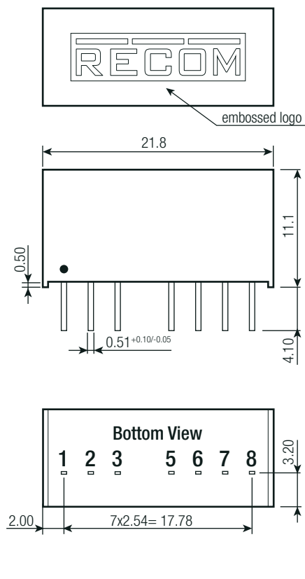
Dimension Drawing (mm)
