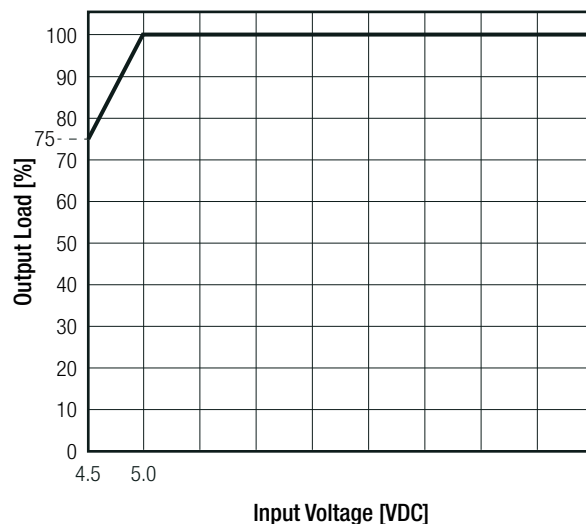
Line Derating
