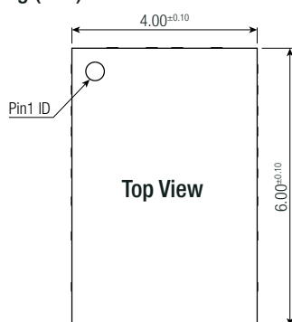
Dimension Drawing (mm)
