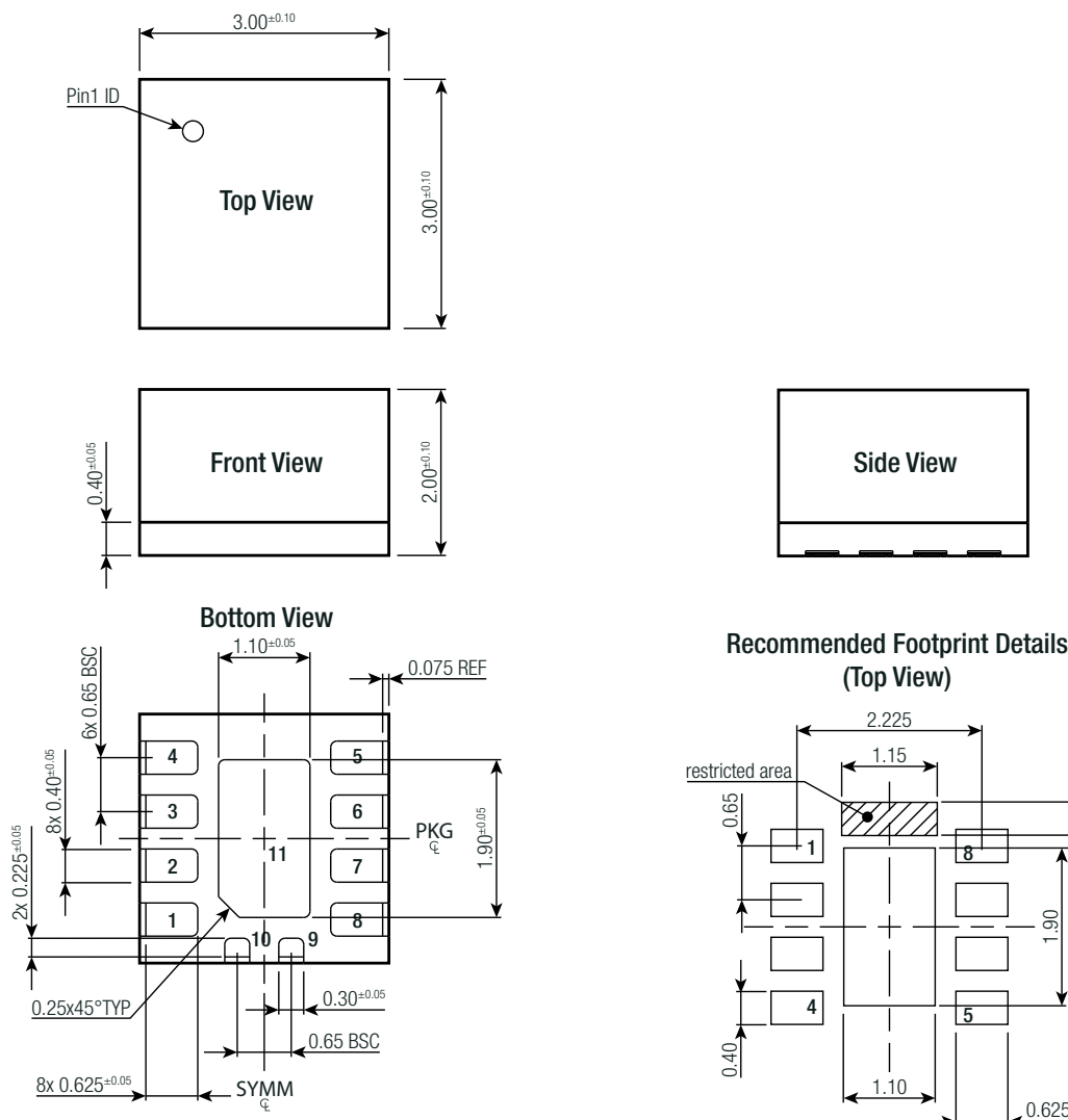
Dimension Drawing (mm)
