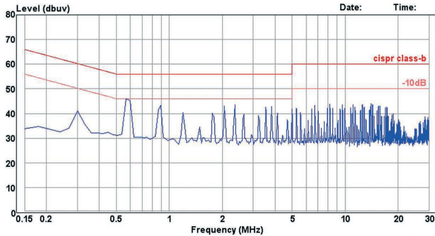
Conducted Emission EN55032 Class B
