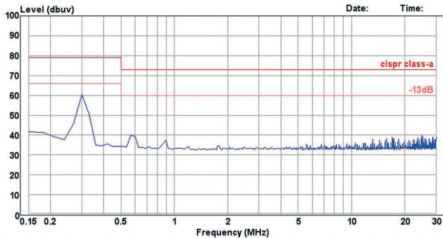
Conducted Emission EN55032 Class A
