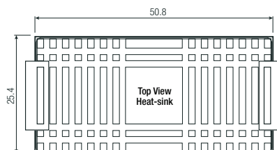
Dimension Drawing with Heat-sink (mm)
