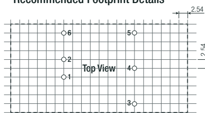
Recommended Footprint Details
