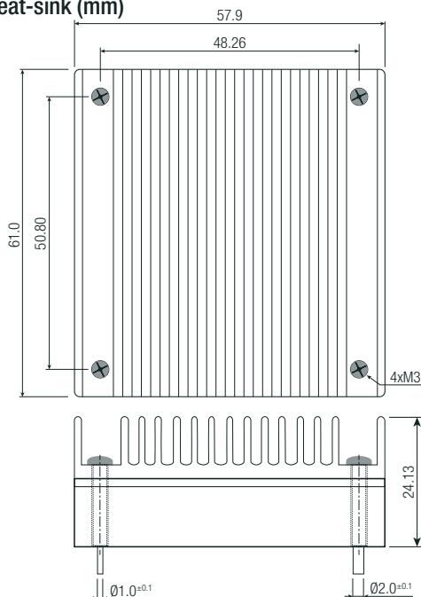
Dimension Drawing Heat-sink (mm)
