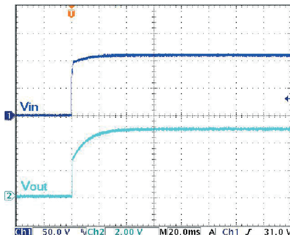
Power up Start-up Characteristic
