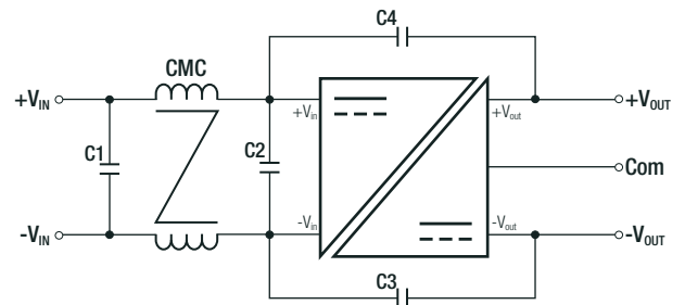
Dual output
