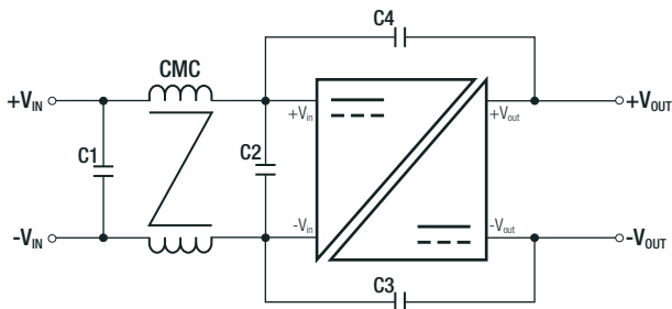
Single output
