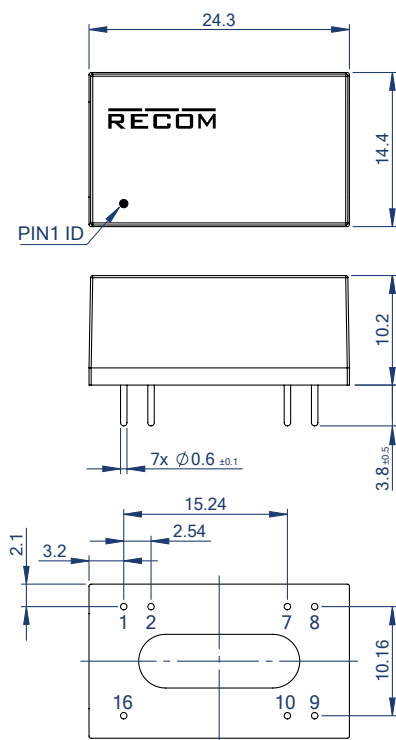
Dimension Drawing DIP16
