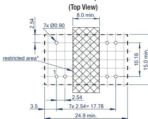
Recommended Footprint Details
