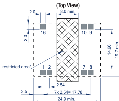
Recommended Footprint Details
