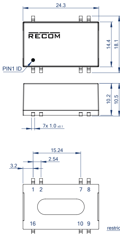
Dimension Drawing SMD
