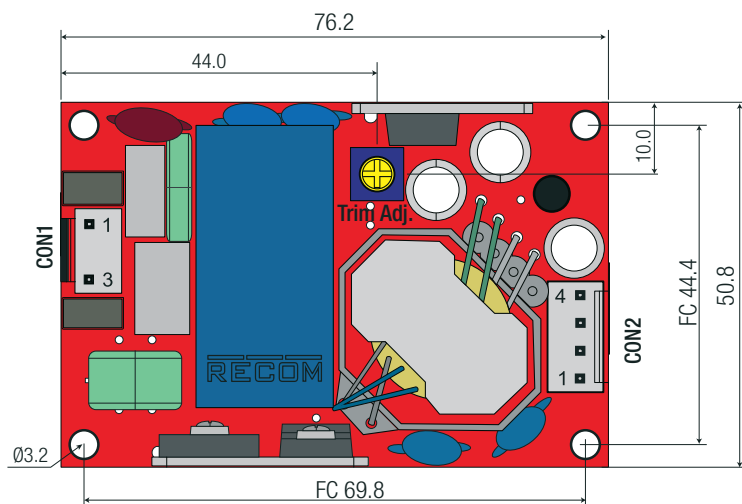
Dimension Drawing Open Frame (/OF) (mm)
