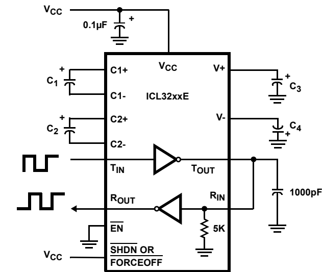
FIGURE 10. TRANSMITTER LOOPBACK TEST CIRCUIT
