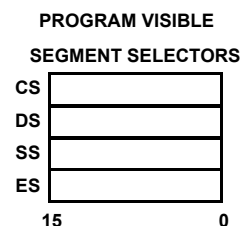
SEGMENT REGISTERS (LOADED BY PROGRAM)
