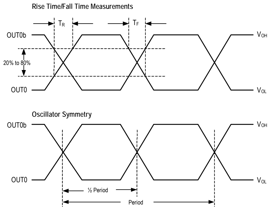
Figure 4. HCSL Output Waveforms
