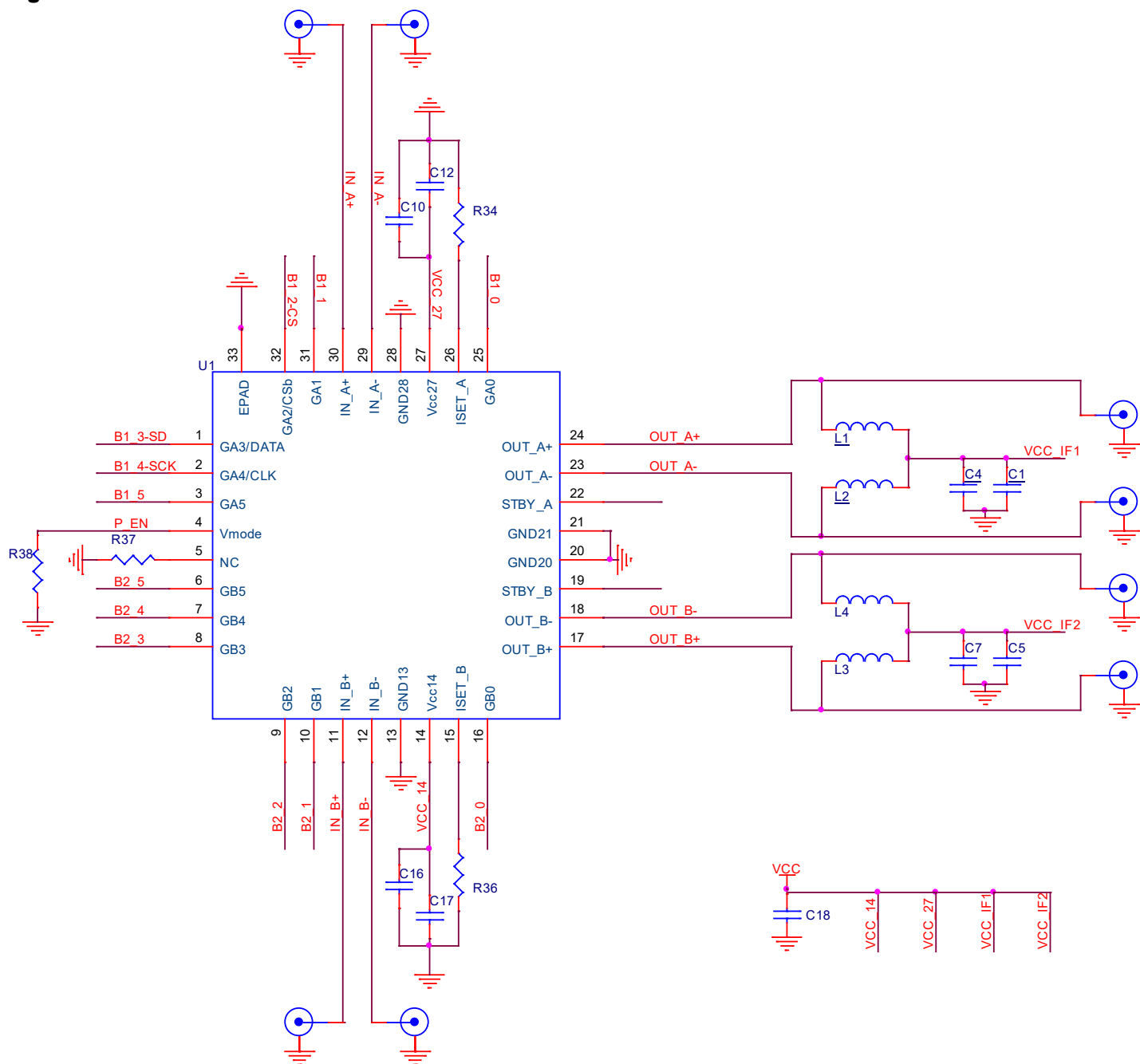
Figure 43. Electrical Schematic
