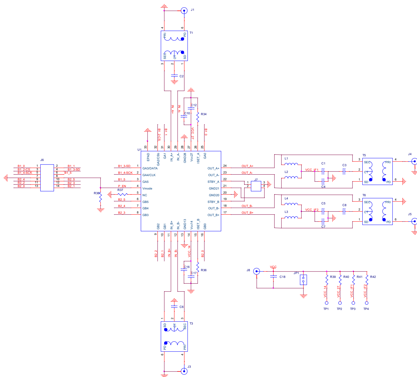
Figure 46. Electrical Schematic
