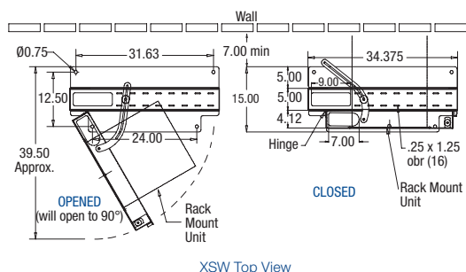
XSW Top View
