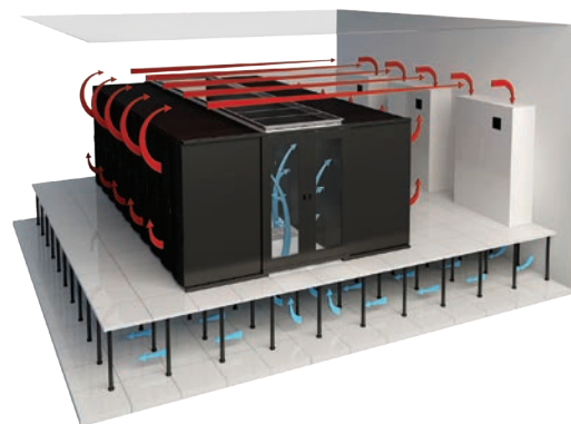
Cold-Aisle Horizontal Design
