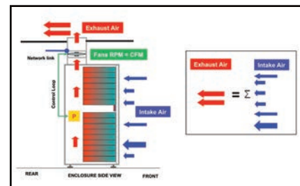
AEHC single cabinet diagram (side view)
