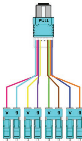
FX Hydra Assembly Type A Polarity MPO-12 8 Fiber
