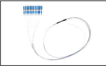
FT3LC250PR12, FX Mass-Fusion Color-coded Pigtail Kit, 12 x LC Simplex on 2m of OM3 ribbon fiber
