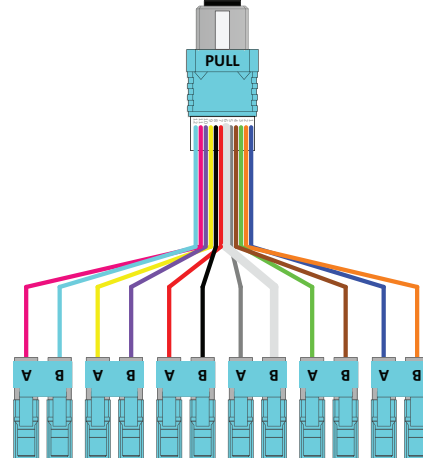
FX Hydra Assembly Type A Polarity MPO-12 12 Fiber
