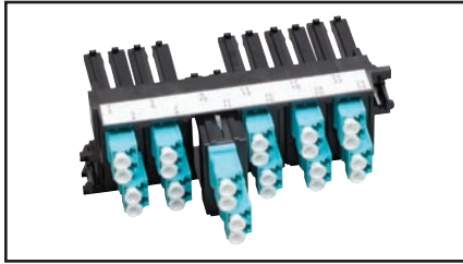
FF3U12LD, FX Ultra Frame, OM3, 12 ports, LC Duplex, Aqua adapters
