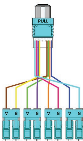
FX Hydra Assembly SR4 Polarity MPO-12 8 Fiber
