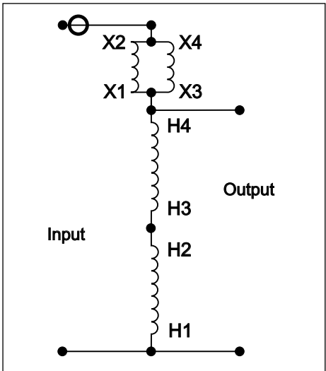
Diagram C2 – Bucking
