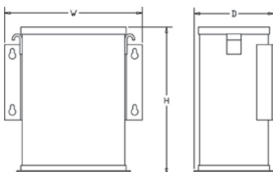
Style 5 - Encapsulated
