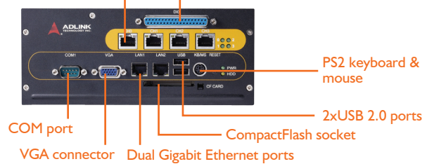
EOS-I000 Front View
