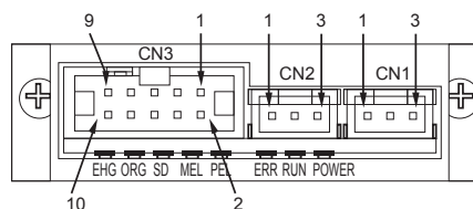
CN1/CN2 Pin Assignment
