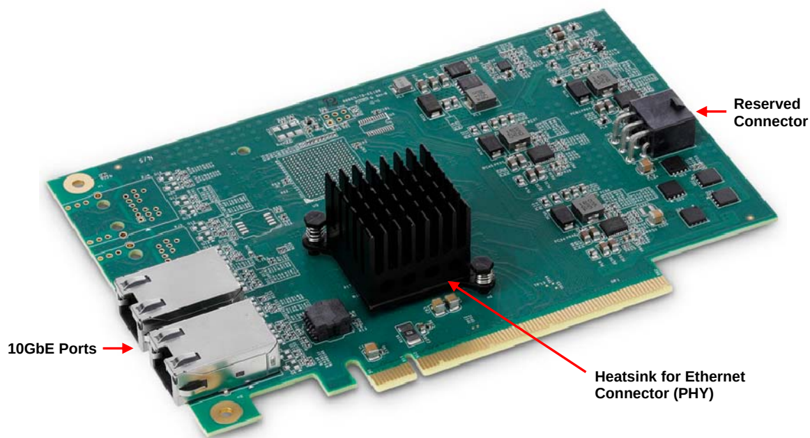
Figure 3: 10GbE BASE-T Card Layout
