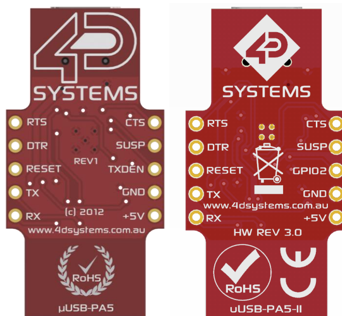
microUSB (μUSB-PA5) additional Pin Outs
