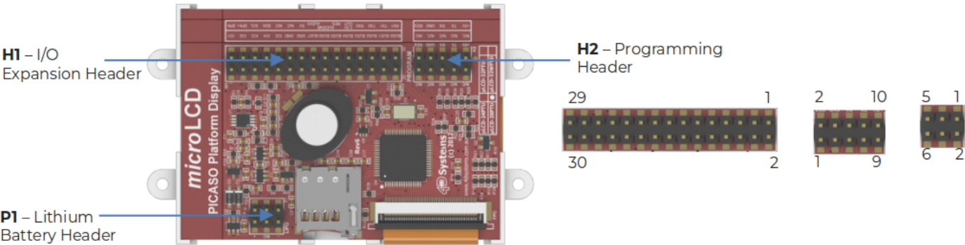
H2 Pinout (Programming Header)
