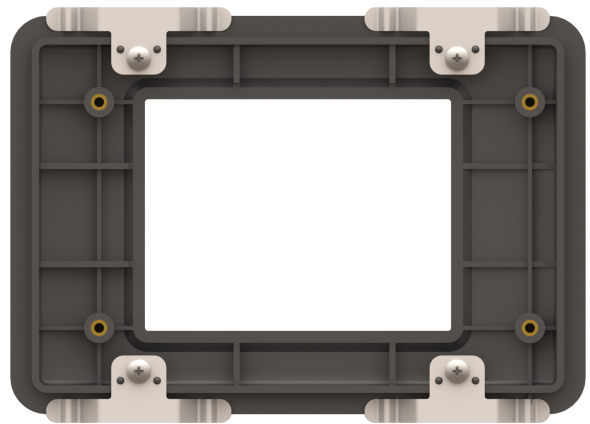
Bare 2.4" Bezel with clips attached - Back
