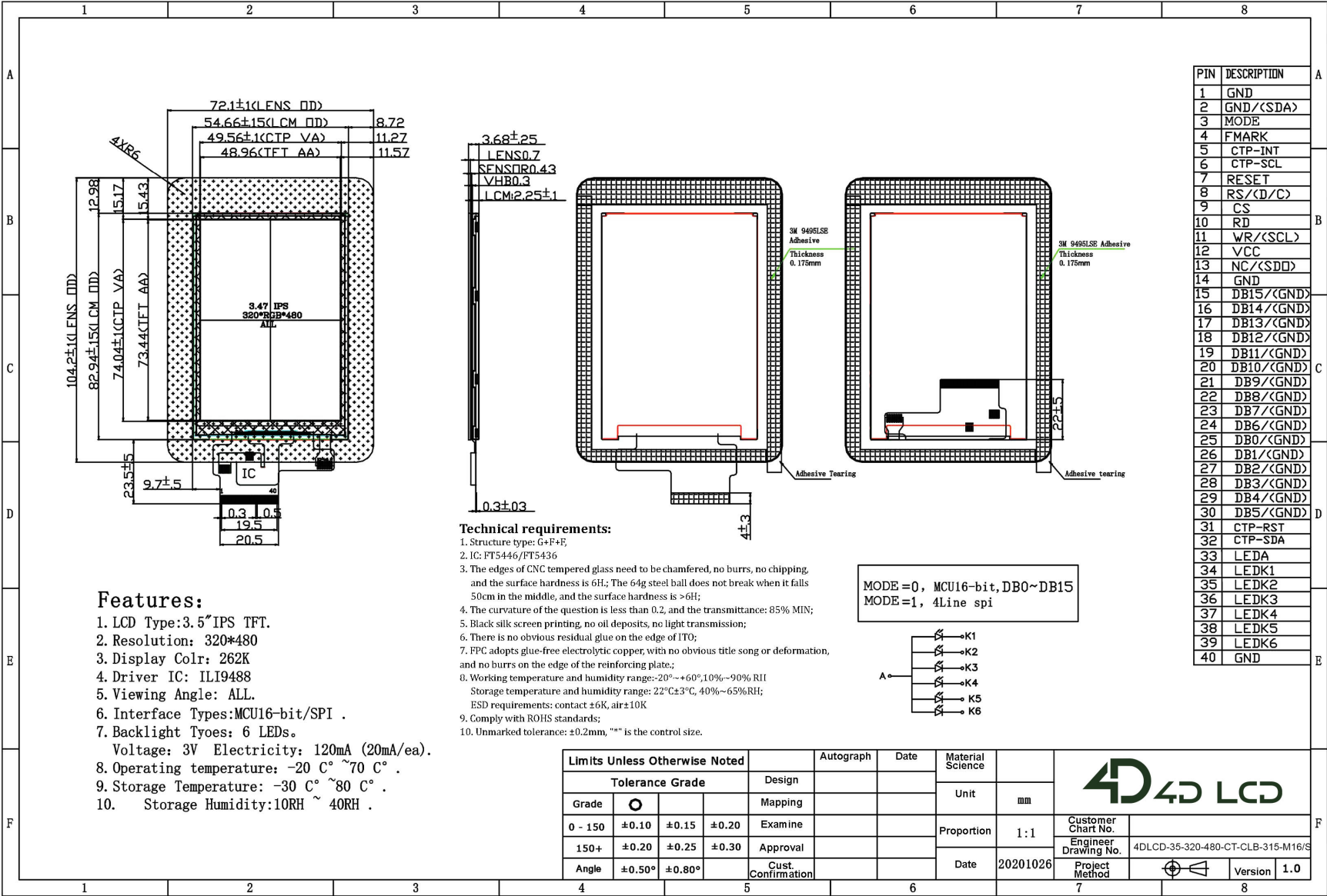
3.5 TFT LCD Display Drawing (Capacitive Touch Version with Cover Lens Bezel)
