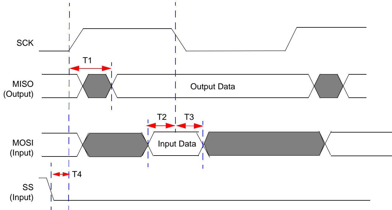
Figure 66. SPI Slave Mode Timing
