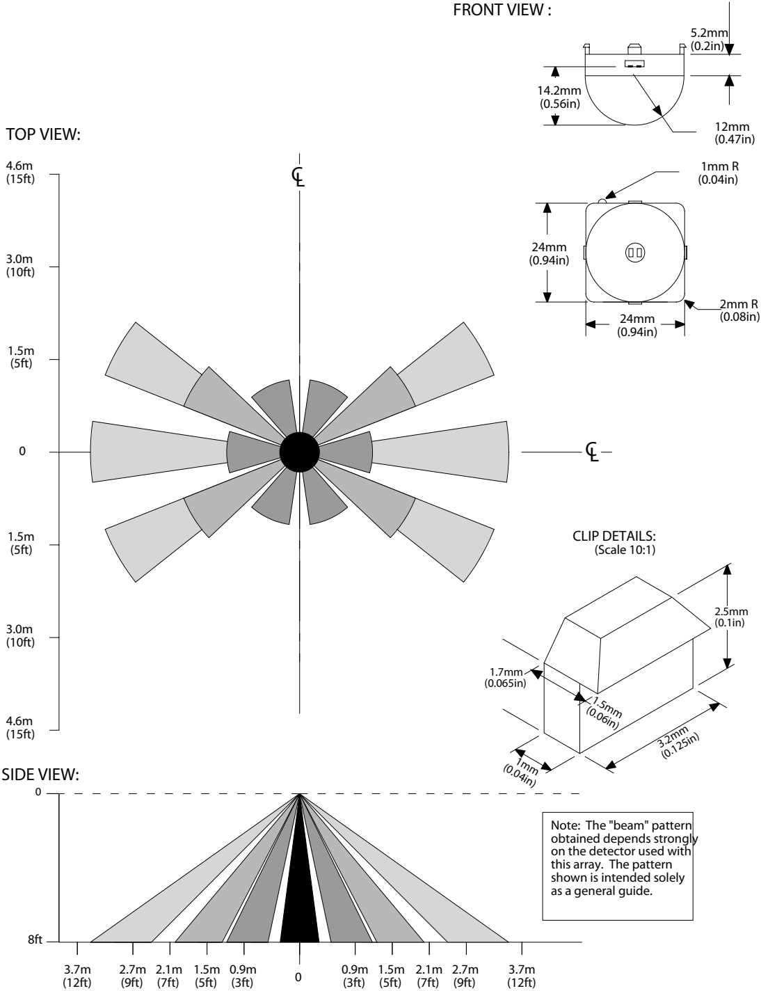
Figure 10. The ZCWM05GIV1 Lens Specification: Ceiling Mount, #1 of 2
