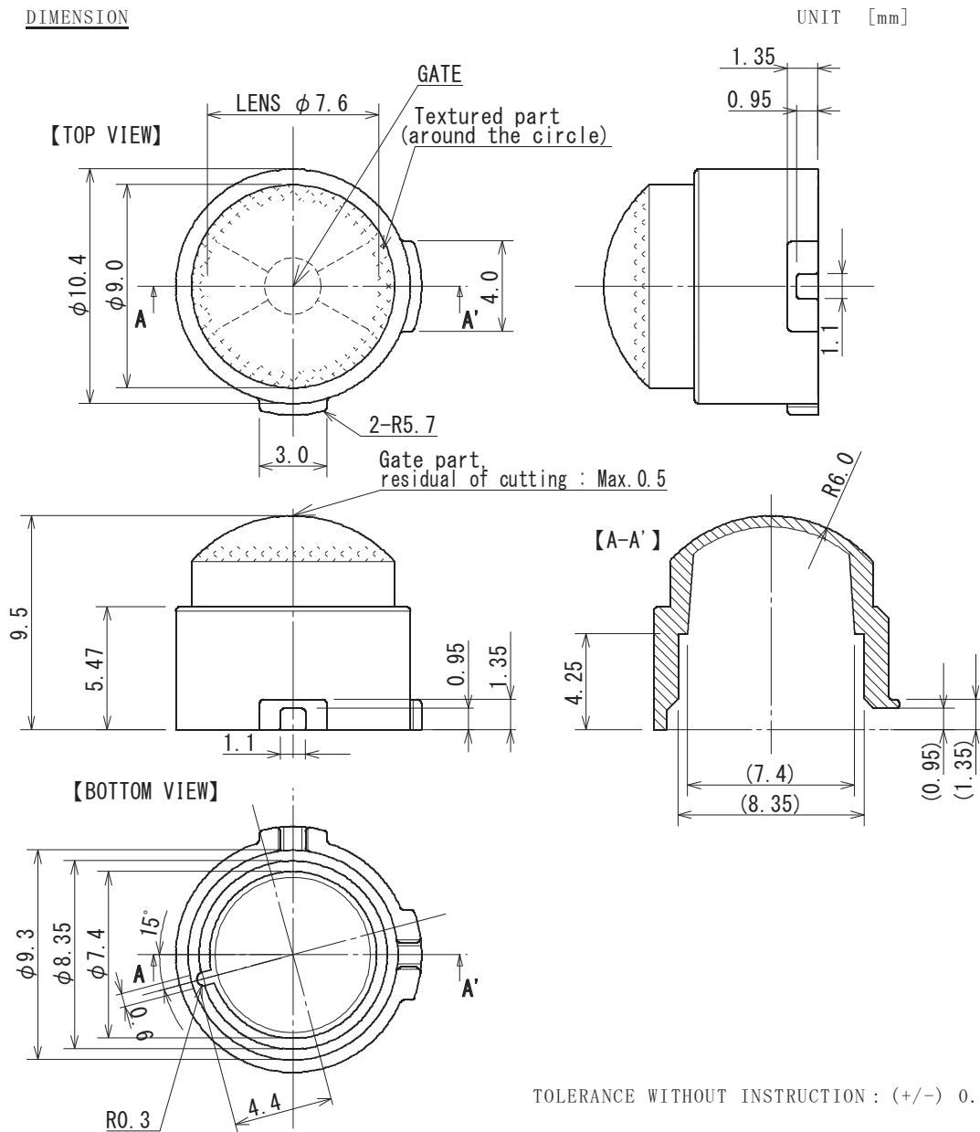
Figure 16. The ZNCL10R Lens Specification, Dimensions
