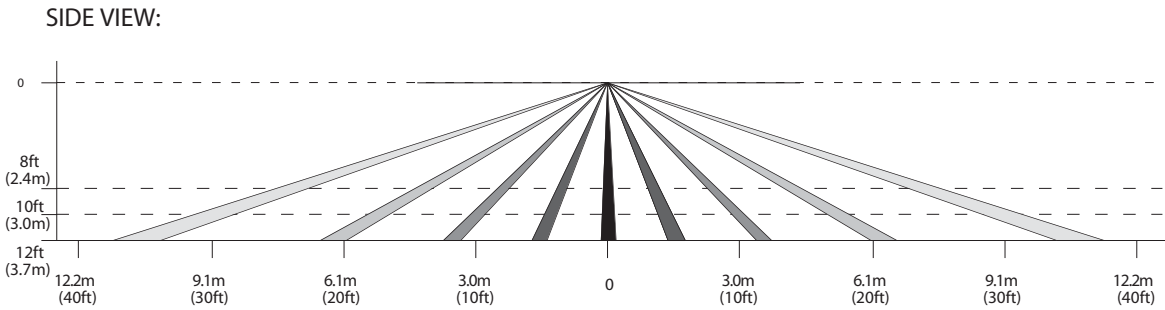
Figure 3. The ZCM077GIV2 Lens Specification: Floor Coverage, Side View
