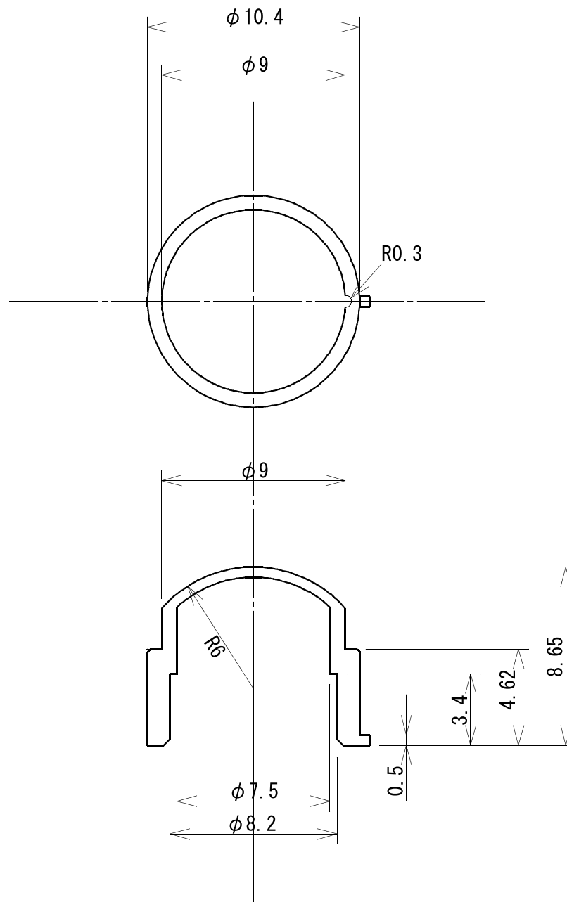
Figure 13. The ZNCL3B Lens Dimensions
