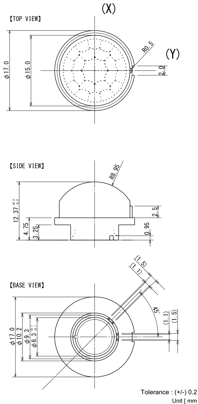
Figure 20. The ZNCL926 Lens Specification, Dimensions
