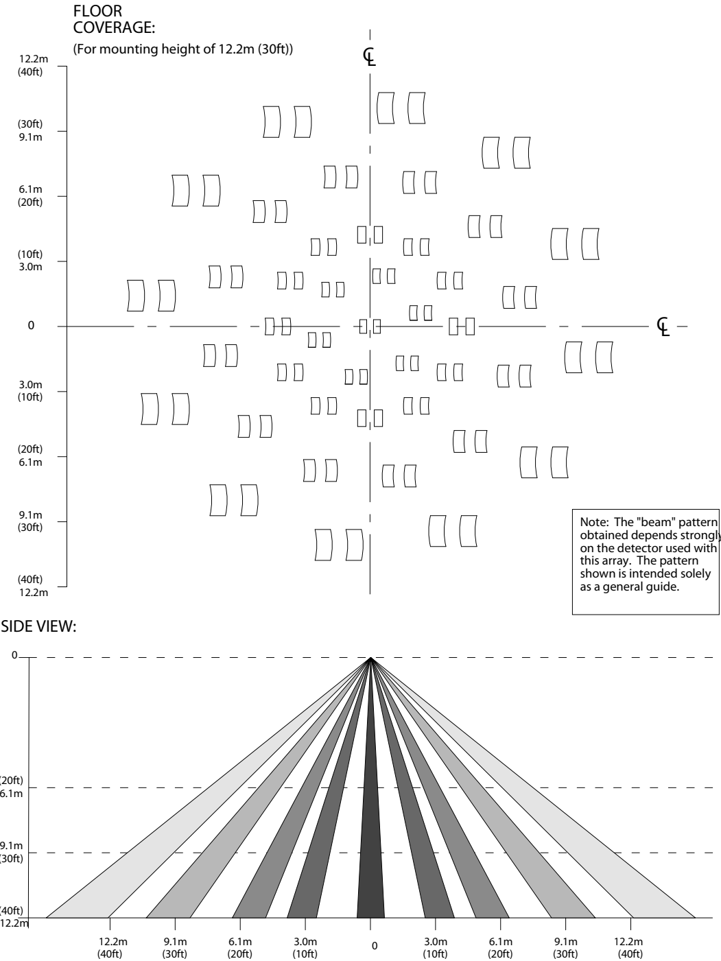
Figure 7. The ZCM077GIV5 Lens Specification, #2 of 3
