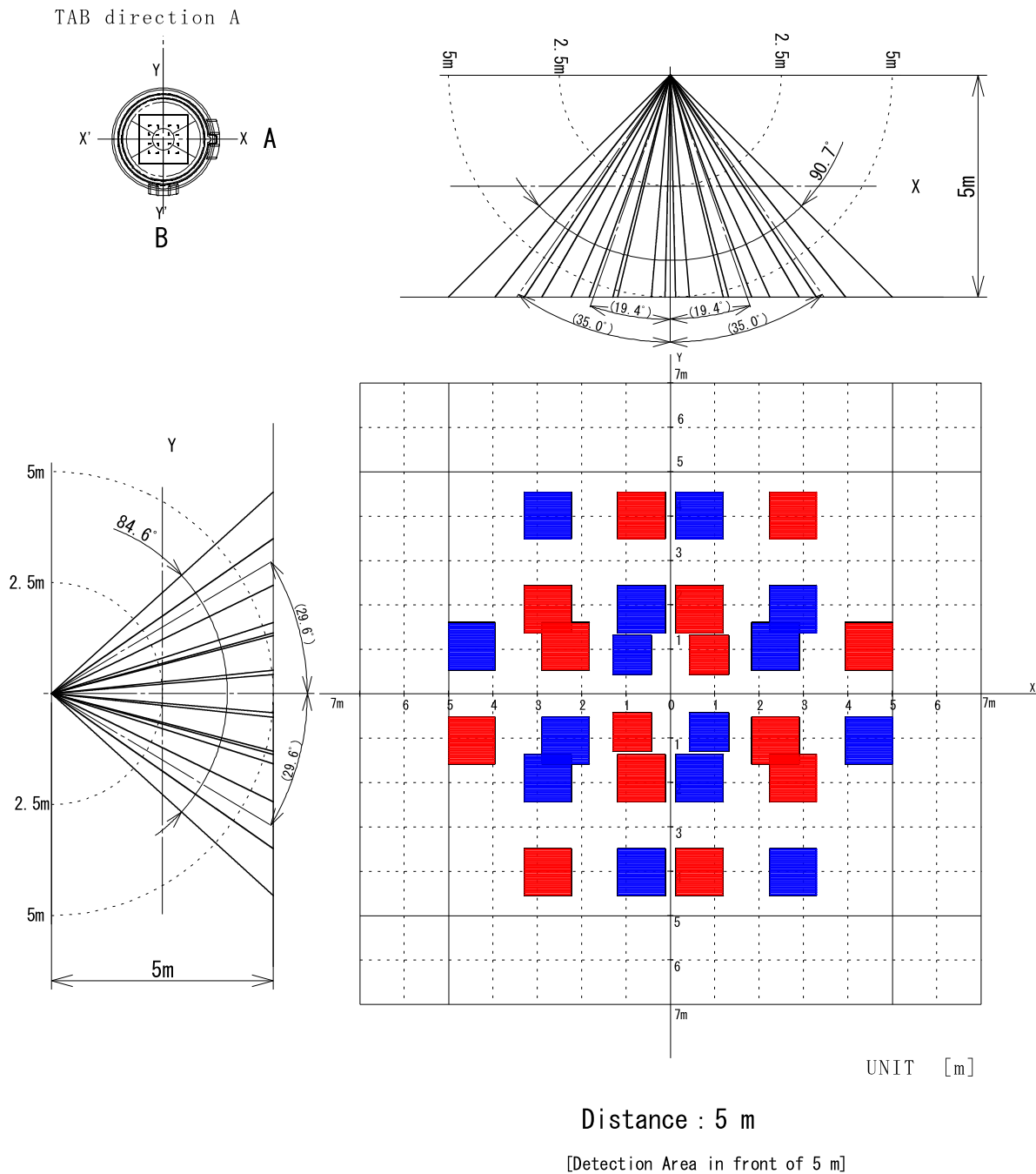
Figure 19. The ZNCL10R Quad-Element Lens Specification, Tab Direction A, X Axis
