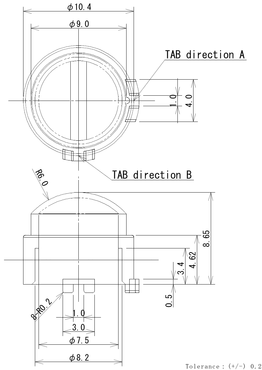
Figure 23. The ZNCL10IL Lens Specification, Dimensions
