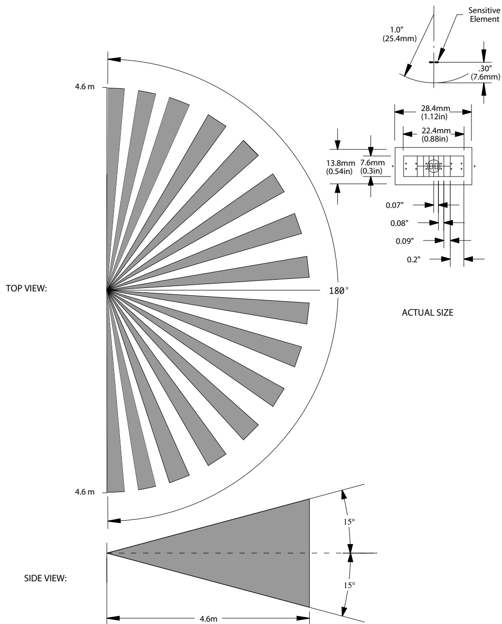
Figure 12. The ZEWA03GIV2 Lens Specification, Dimensions
