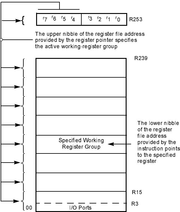
Figure 17. Register Pointer—Detail
