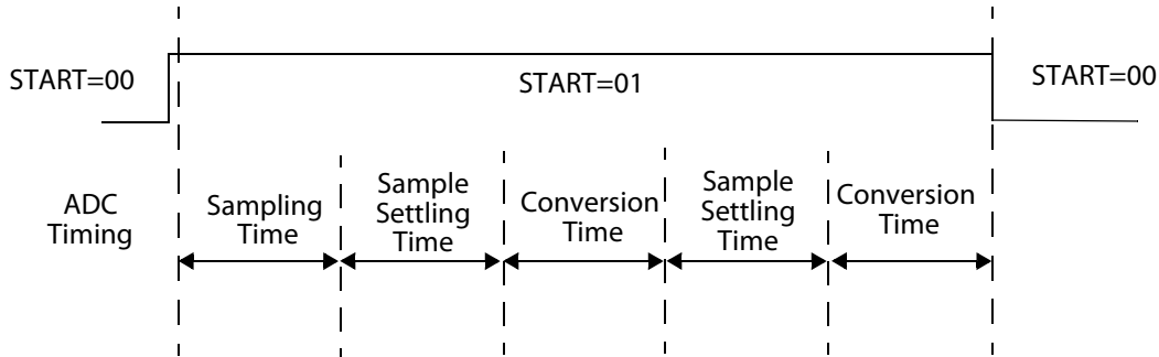
Figure 75. ADC Timing Diagram for 2-Pass 14-Bit Resolution with INMODE=10, 11
