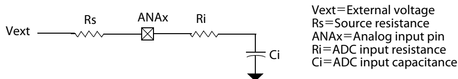
Figure 77. ADC Input Equivalent Circuit
