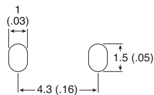
Mounting Holes
