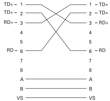
Wiring Diagram for Y-ConJack-25
