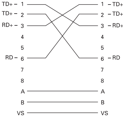
Wiring Diagram for Y-ConJack-26C
