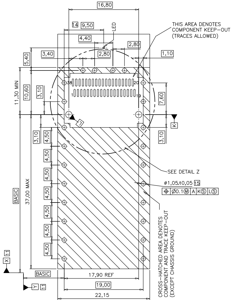
RECOMMENDED DOUBLE SIDE PC BOARD LAYOUT
