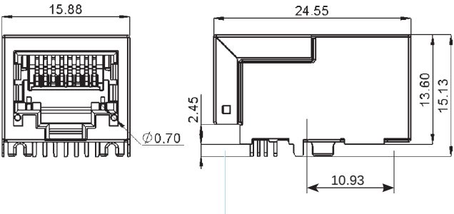
Y-ConJack-31
