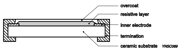
Fig. 10 Chip resistor outlines
