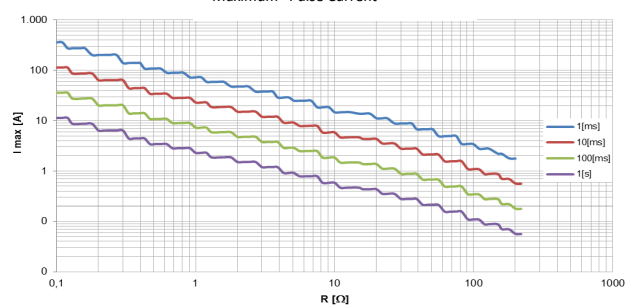
Maximum Pulse Current
