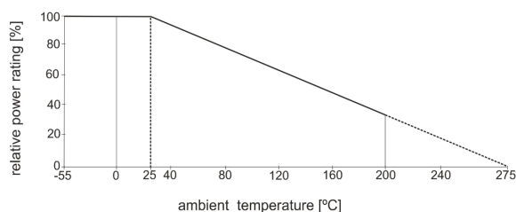
Derating – P 25
