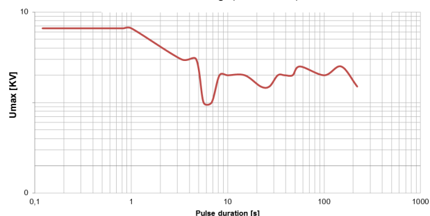
Maximum Pulse Voltage (IEC61000-4-5)
