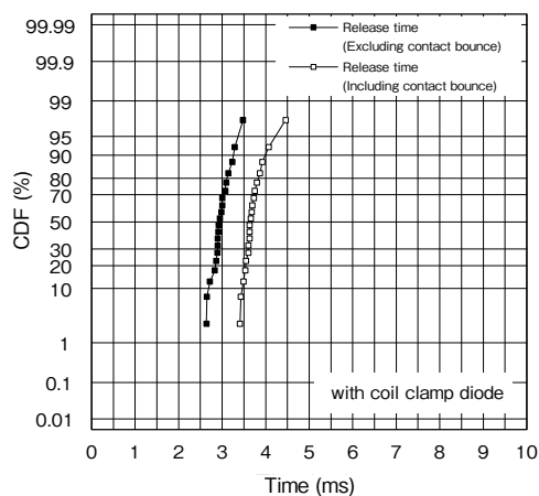
Release Time
