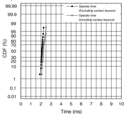
Operate Time
