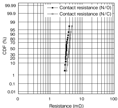
Contact Resistance
