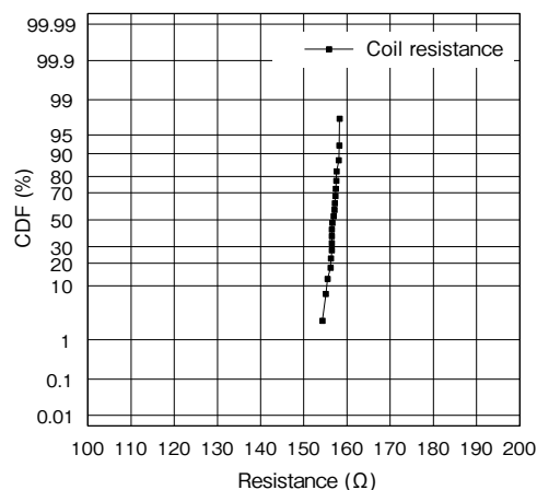
Coil Resistance
