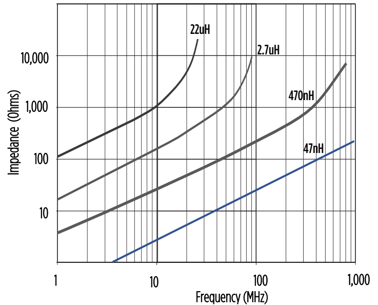
Typical Impedance vs Frequency
